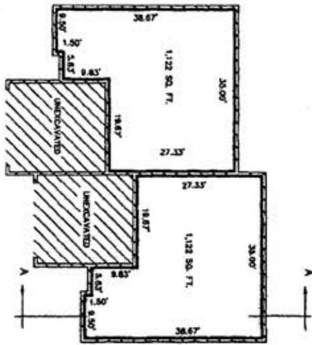
BASEMENT PLAN
